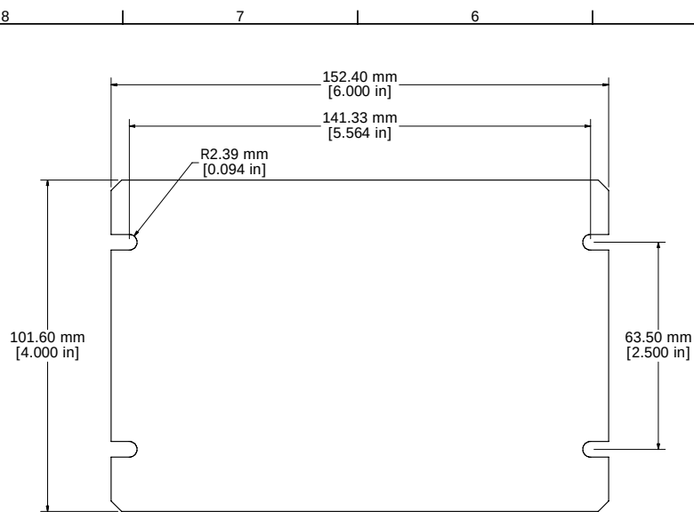
1431-8 OR 1431-8BK3 - VIEW FROM TOP (SOLD SEPERATELY)
