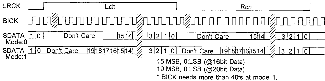
Figure 3. Digital Input Formats 0 &amp; 1
