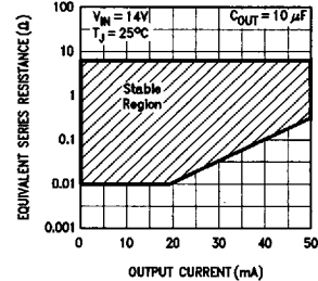
Output Capacitor ESR
