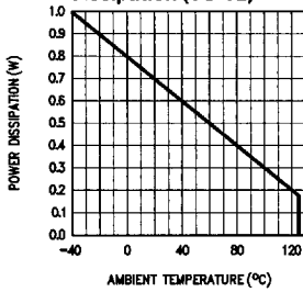
Maximum Power Dissipation (TO-92)
