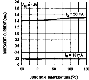
Quiescent Current
