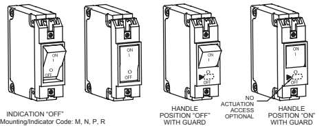
MARKING DETAIL "C" (SEE TABLE)
