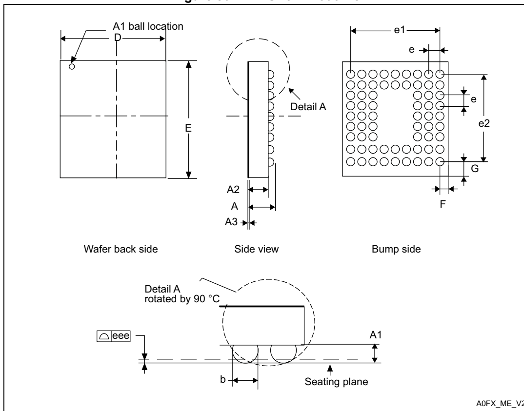
Figure 80. WLCSP64+2 outline
