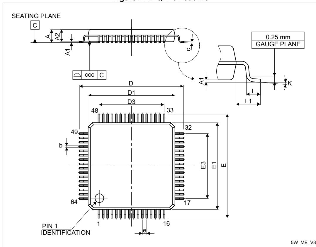
Figure 77. LQFP64 outline
