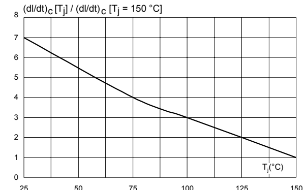
Figure 12. Relative variation of critical rate of decrease of main current (di/dt)_c versus junction temperature (typical values)
