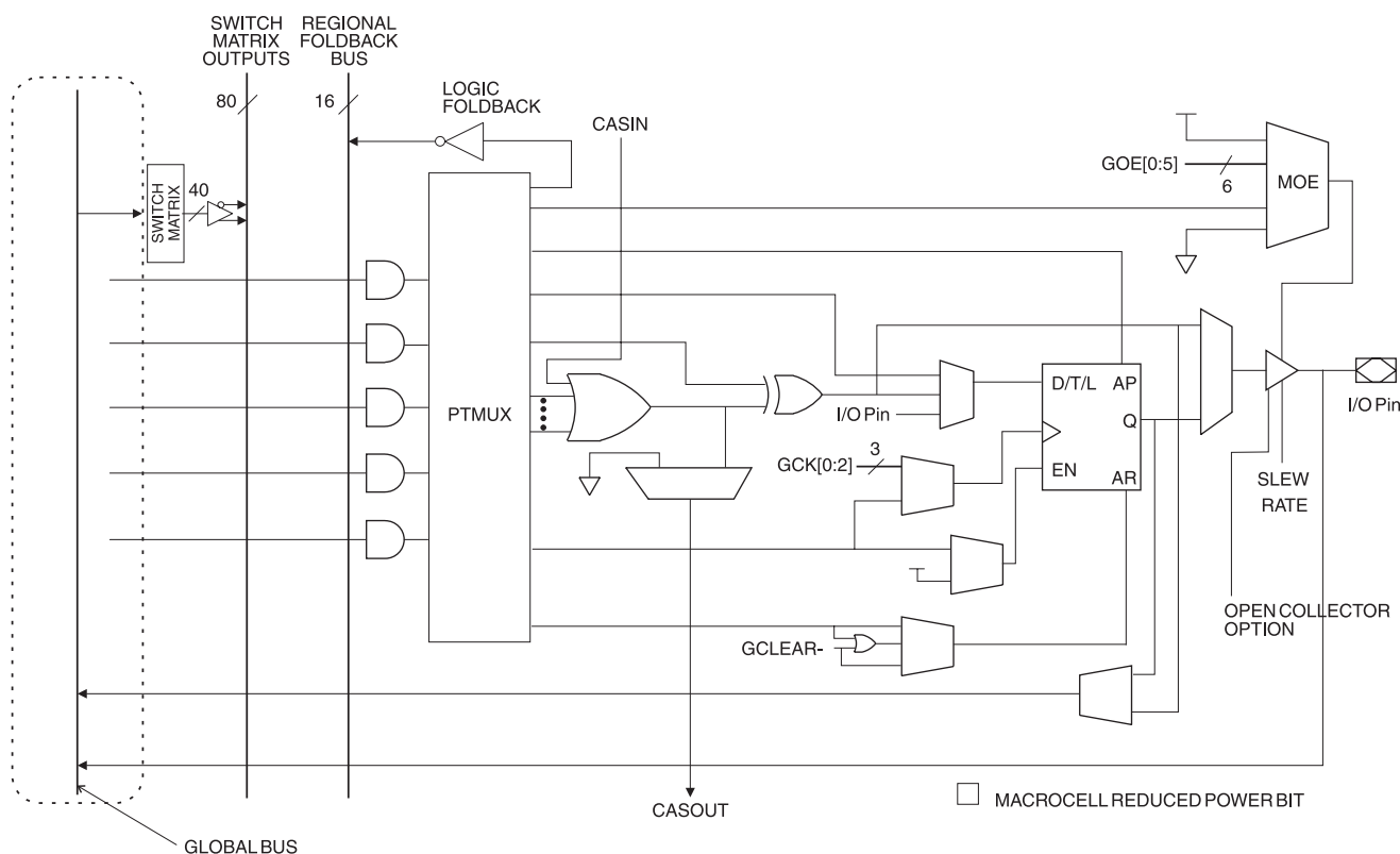
Figure 1. ATF1508ASV(L) Macrocell
