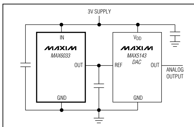
Figure 2. 14-Bit High-Resolution DAC and Positive Reference from a Single 3V Supply
