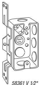
58361 V 1/2* CV bracket recessed ½"
