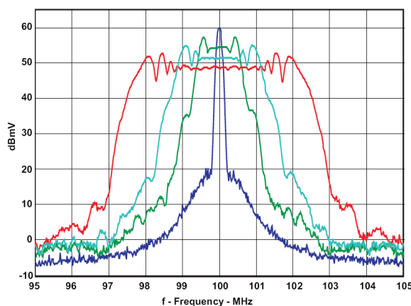
CDCE502 with a 25MHz Crystal, FS = 1, f_{OUT} = 100MHz, and 0%, \pm 0.5 , \pm 1\% , and \pm 2\% SSC
