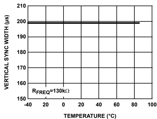
FIGURE 33. VERTICAL SYNC WIDTH vs TEMPERATURE
