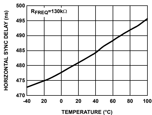
FIGURE 28. HORIZONTAL DELAY vs TEMPERATURE
