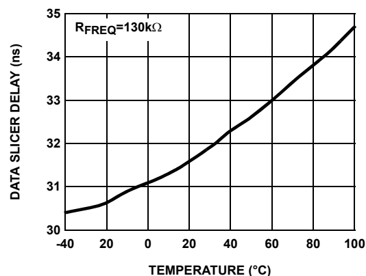
FIGURE 29. DATA SLICER DELAY vs TEMPERATURE - DS MODE = 1
