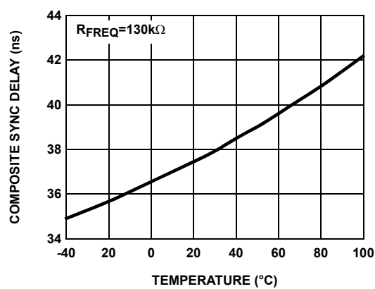
FIGURE 26. COMPOSITE DELAY vs TEMPERATURE - FSEL = 0
