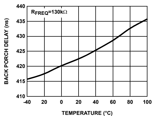
FIGURE 31. BACK PORCH DELAY vs TEMPERATURE - FSEL = 1
