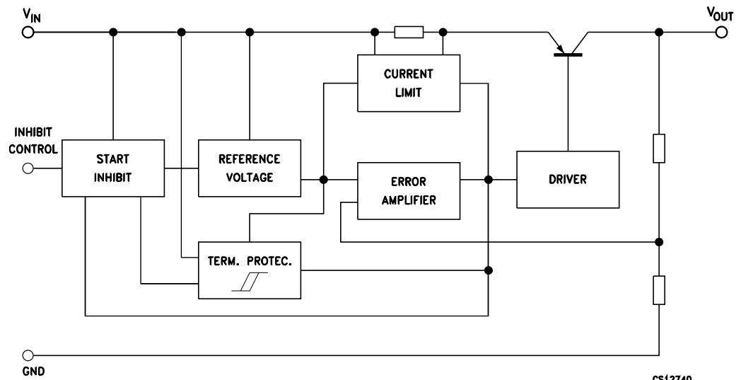
Figure 1. Schematic diagram
