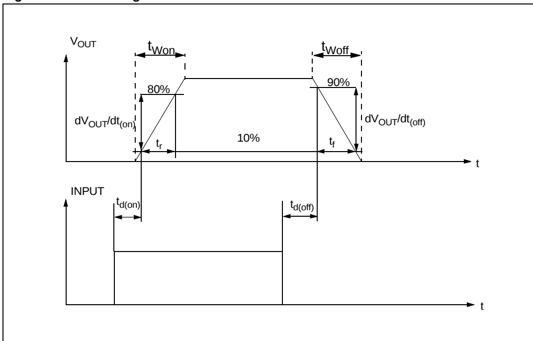
Figure 6. Switching characteristics
