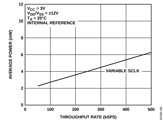
Figure 48. Power vs. Throughput Rate with 3 V V CC
