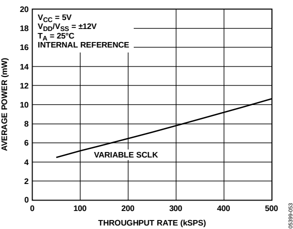
Figure 49. Power vs. Throughput Rate with 5 V V CC
