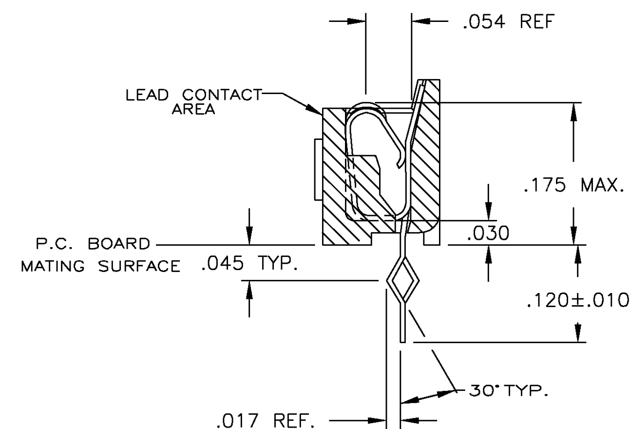
SECTION A-A ROTATED 90° CW SCALE 10:1 FOR -6, -7 & -8 ONLY
