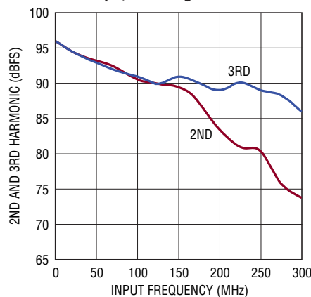
LTC2164: 2nd, 3rd Harmonic vs Input Frequency, -1\text{dBFS} , 105\text{Mpsps} , 1\text{V} Range
