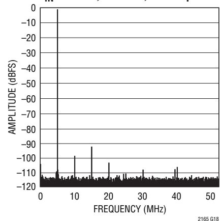
LTC2164 64k Point FFT, f_{IN} = 5\text{MHz} , -1dBFS, 105Msps
