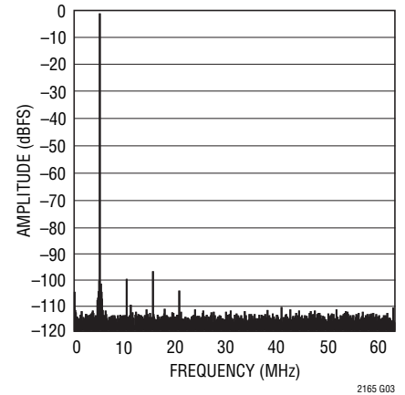
LTC2165 64k Point FFT, f_{IN} = 5\text{MHz} , -1dBFS, 125Msps
