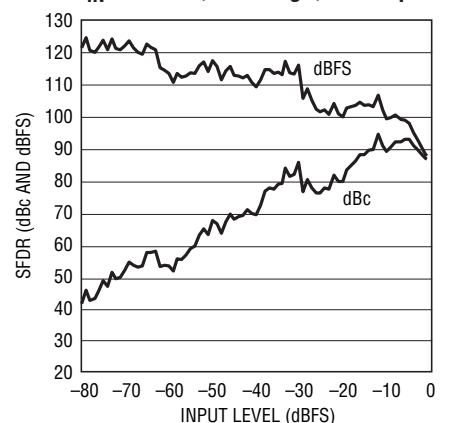
LTC2164 SFDR vs Input Level, f_{IN} = 70\text{MHz} , 2\text{V} Range, 105\text{Mpsps}
