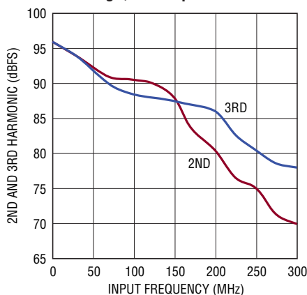
LTC2164 2nd, 3rd Harmonic vs Input Frequency, -1\text{dBFS} , 2\text{V} Range, 105\text{Mpsps}
