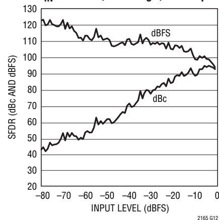
LTC2165 SFDR vs Input Level, f_{IN} = 70\text{MHz} , 2V Range, 125Msps
