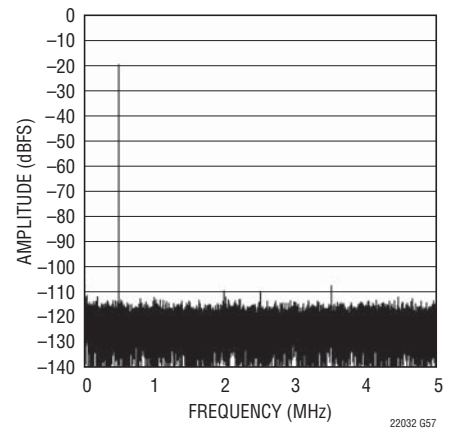
LTC2202: 32K Point FFT, f_{IN} = 30.5\text{MHz} , -20\text{dBFS} , PGA = 1
