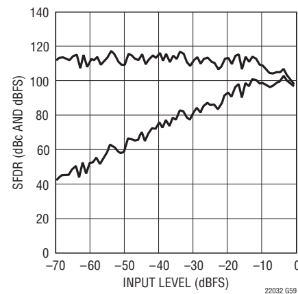
LTC2202: SFDR vs Input Level, f_{IN} = 30.1\text{MHz} , PGA = 0, Dither "On"
