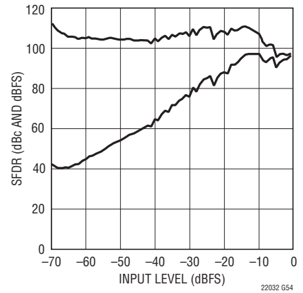
LTC2202: SFDR vs Input Level, f_{IN} = 12.4\text{MHz} , PGA = 0, Dither "Off"
