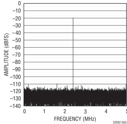
LTC2202: 32K Point FFT, f_{IN} = 12.4\text{MHz} , -20\text{dBFS} , PGA = 0
