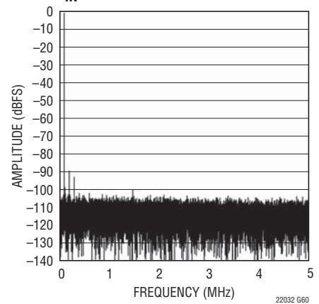
LTC2202: 32K Point FFT, f_{IN} = 70.1\text{MHz} , -1\text{dBFS} , PGA = 1
