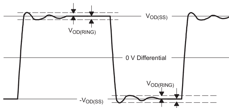
Figure 3. V_{OD}(\text{RING}) Waveform and Definitions
