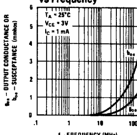
Typical Output Admittance vs Frequency
