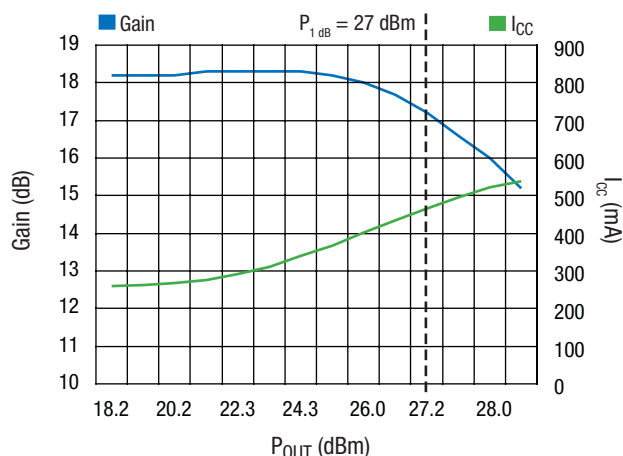
SKY65112 Gain, I_{CC} vs. P_{OUT} V_{CC} = 5\text{ V} , V_{REF} = 5.1\text{ V} , I_{CCQ} = 260\text{ mA} , F = 940\text{ MHz}
