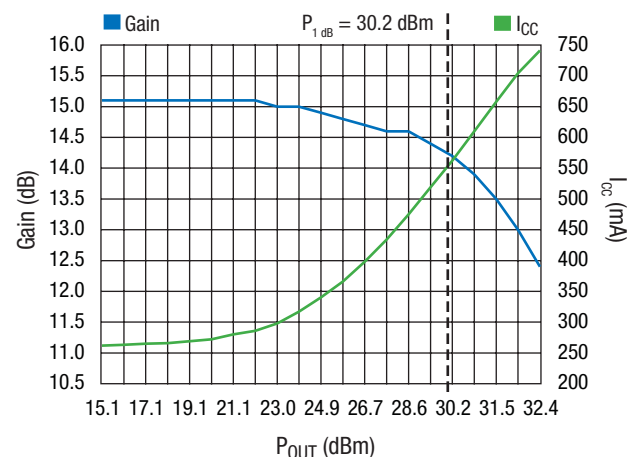
SKY65112 Gain, I_{CC} vs. P_{OUT} V_{CC} = 5\text{ V} , V_{REF} = 5\text{ V} , I_{CCQ} = 260\text{ mA} , F = 1960\text{ MHz}
