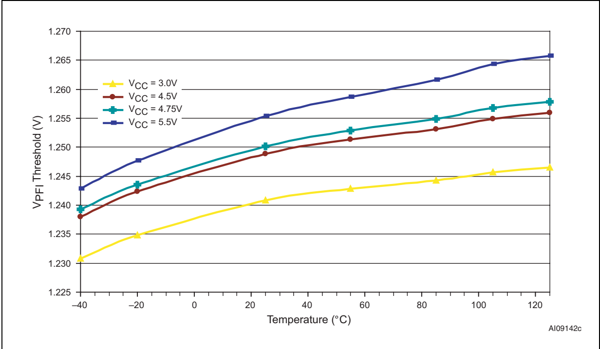
Figure 21. V_{PFI} threshold vs. temperature
