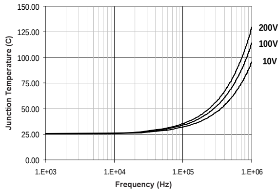
Figure 33. IR2010S Tj vs Frequency R GATE = 16 Ohm, V cc = 15V with IRFBC40
