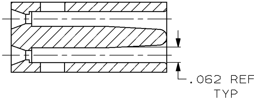
SECT Y-Y
