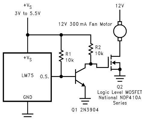
FIGURE 8. Simple Fan Controller, Interface Optional
