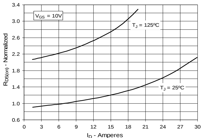
Fig. 5. R_{DS(on)} Normalized to I_D = 7\text{A} Value vs. Drain Current
