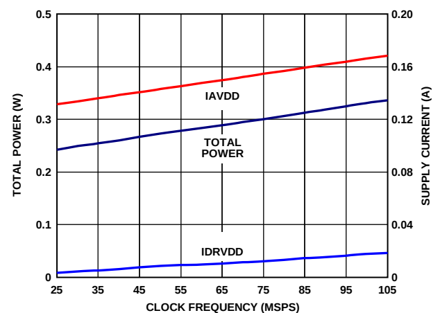
Figure 82. AD9255-105 Power and Current vs. Sample Rate
