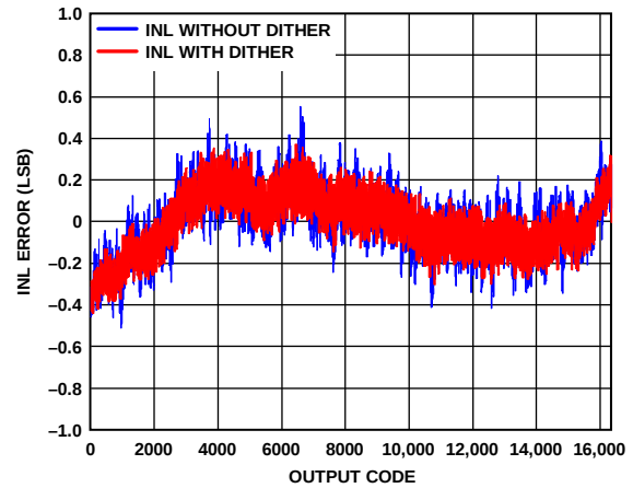
Figure 16. AD9255-80 INL with f_{IN} = 12.5 MHz
