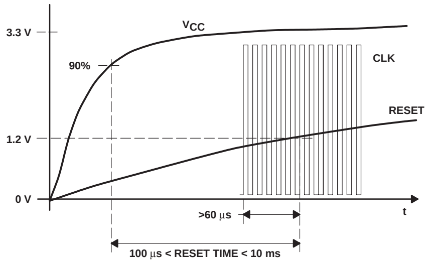
Figure 4-6. Reset Timing
