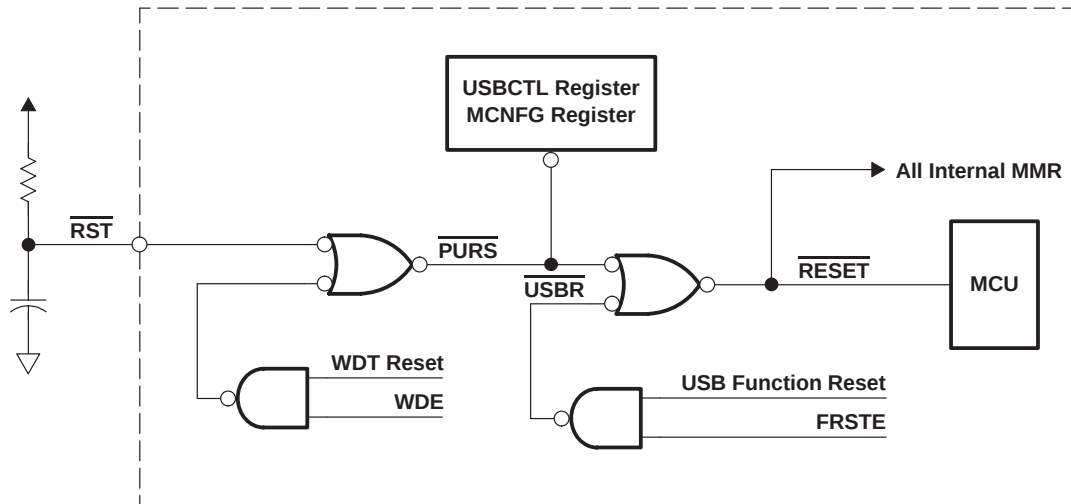
Figure 2–2. Reset Diagram
