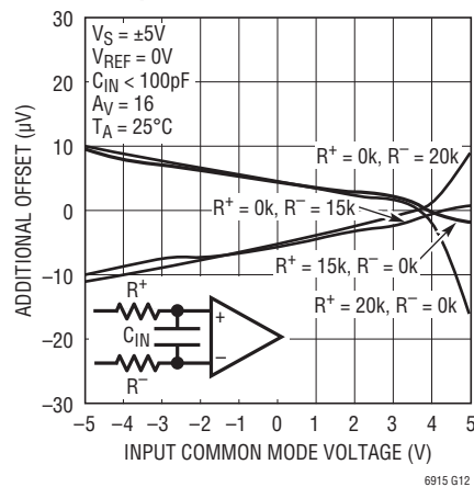
Error Due to Input R_S Mismatch vs Input Common Mode
