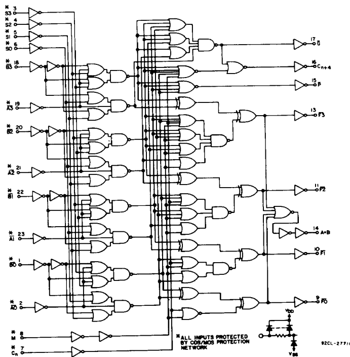
Fig. 3 – CD40181B logic diagram (active-low data).
