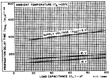
Fig. 6 – Typical propagation delay time as a function of load capacitance (for A or B to F, logic mode).
