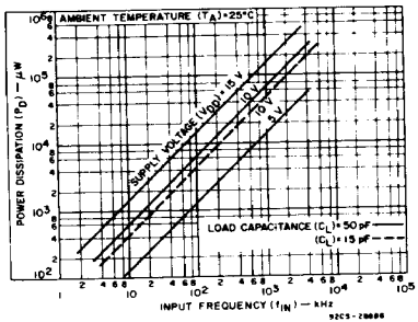
Fig. 8 – Typical dynamic dissipation as a function of input frequency (see Fig. 11 – dynamic power dissipation test circuit).
