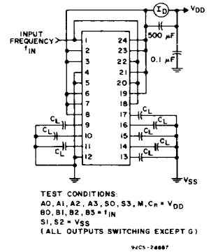
Fig. 11 - Dynamic power dissipation test circuit.
