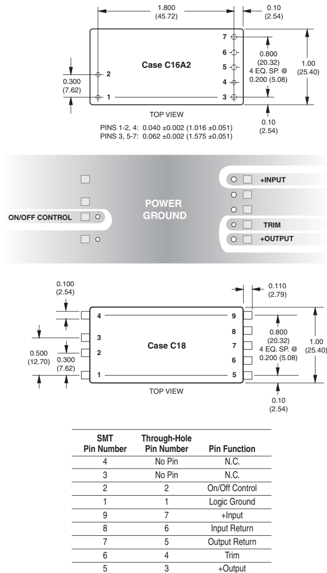
Figure 5. Recommended Board Layout
