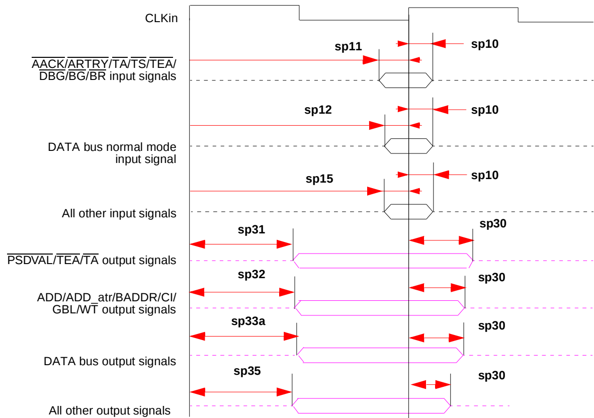
Figure 9. Bus Signals
