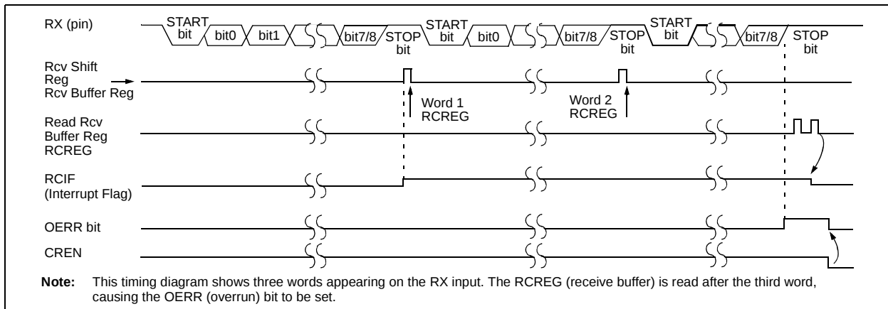
FIGURE 9-5: ASYNCHRONOUS RECEPTION
