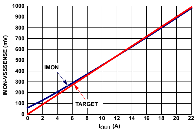
FIGURE 38. IMON, VID = 1.2375
