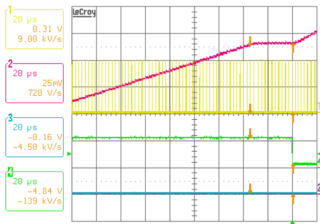
FIGURE 30. CPU MODE CLK\_EN\# DELAY, V_{IN} = 19V , I_O = 0A , V_{ID} = 1.2V , Ch1: PHASE1, Ch2: V_O , Ch4: CLK\_EN\#
