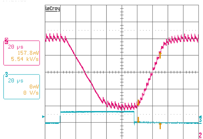
FIGURE 45. CPU MODE VID TRANSITION, DPRSLPVR = 1, I_O = 2A , VID = 1.2375V/1.0375V, Ch2: V_O , Ch3: VID4
