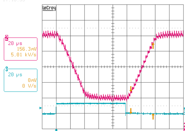
FIGURE 44. GPU MODE VID TRANSITION, DPRSLPVR = 0, I_O = 2A , V_{ID} = 1.2375V/1.0375V , Ch2: V_O , Ch3: V_{ID4}
