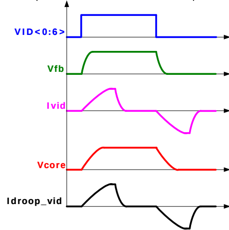
FIGURE 23. OPTIONAL SLEW RATE COMPENSATION CIRCUIT FOR 1-TICK VID TRANSITION
