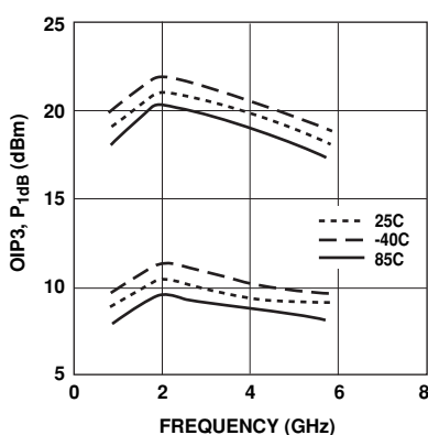
Figure 15. OIP3 and P_{1dB} vs. Frequency and Temperature [1,2] , V_{DS}=2V , I_{DS}=15\text{ mA} .
