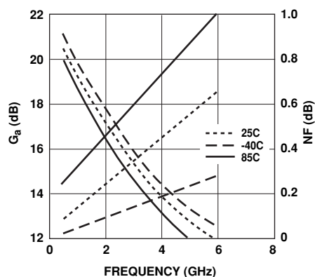
Figure 14. F_{min} and G_a vs. Frequency and Temperature, V_{DS}=2V , I_{DS}=15\text{ mA} .
