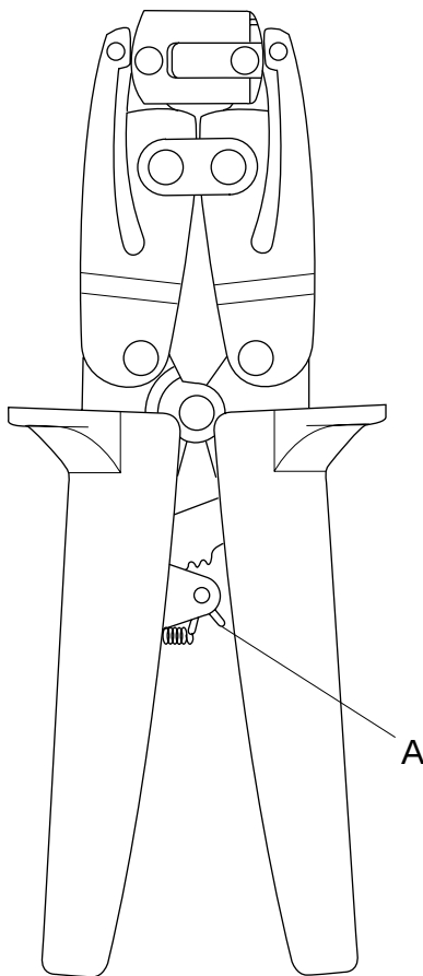
K32GL, K34GL UNIVERSAL FERRULE CRIMPERS
