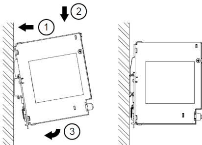
Fig. 6.1 Mounting
