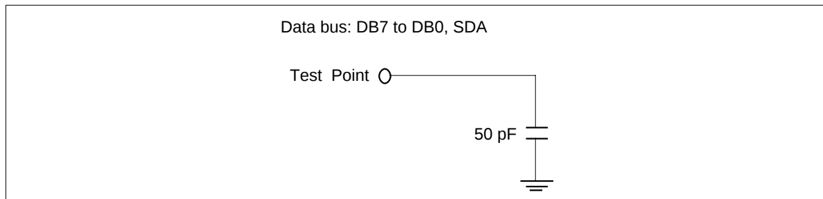
Figure 64 Load Circuit
