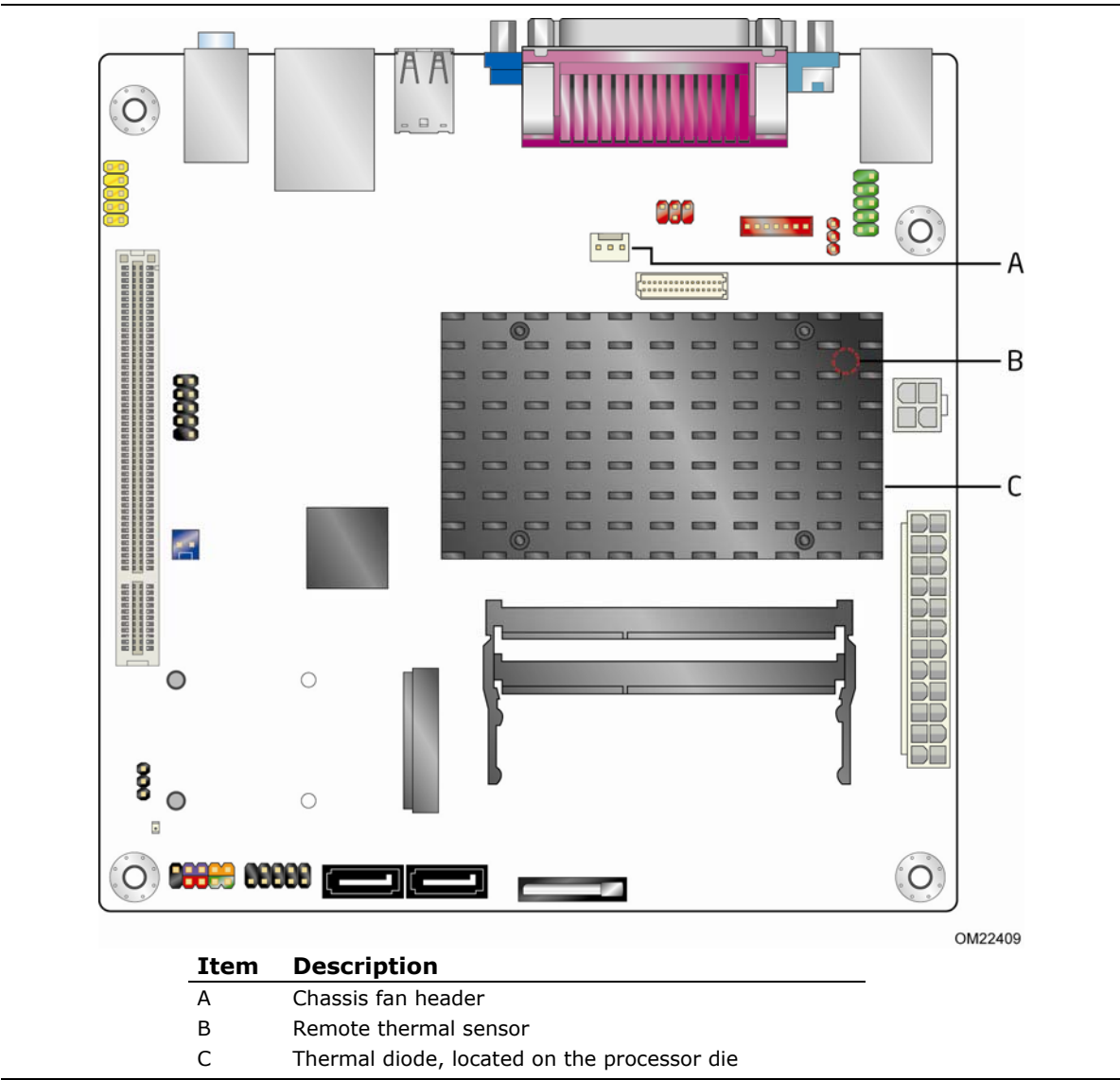
Figure 5. Thermal Sensors and Fan Header
