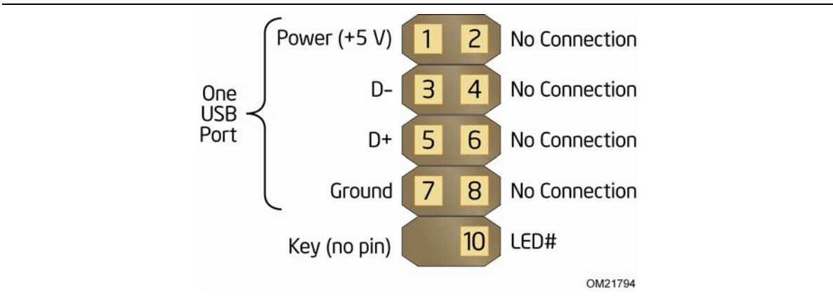
Figure 13. Connection Diagram for Front Panel USB Header with Intel Z-U130 USB Solid-State Drive or Compatible Device Support (D425KTW only)
