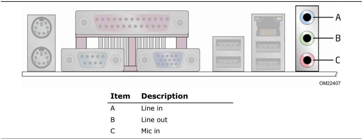
Figure 4. Back Panel Audio Connectors
