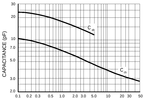
Figure 9. Capacitance
