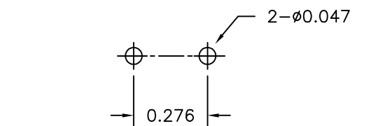
RECOMMENDED MOUNTING PATTERN
