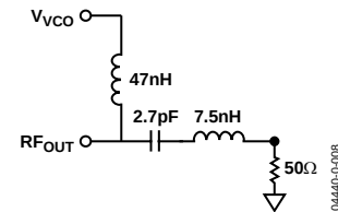
Figure 21. Optimum ADF4360-6 Output Stage
