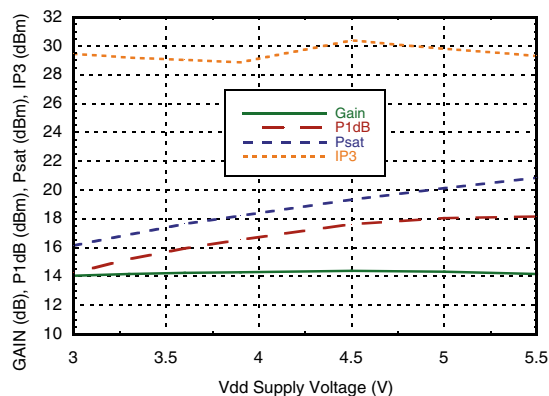
Gain, Power & Output IP3 vs. Supply Voltage @ 10 GHz
