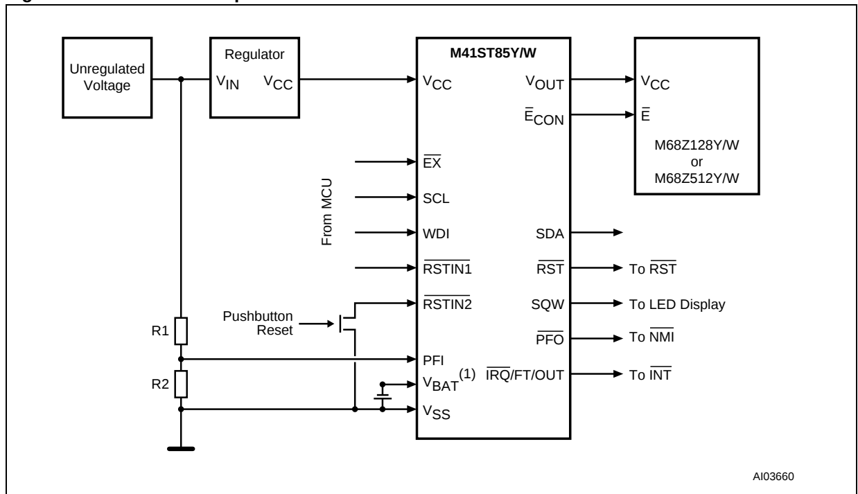
Figure 7. Hardware Hookup
