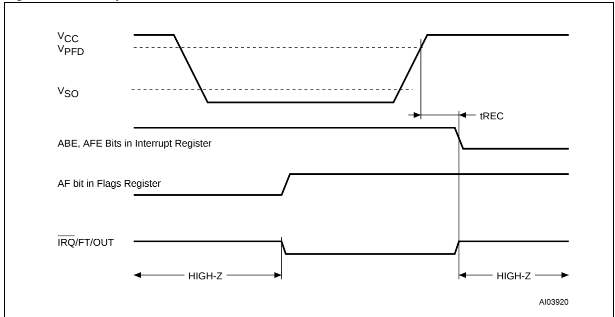
Figure 19. Back-Up Mode Alarm Waveform
