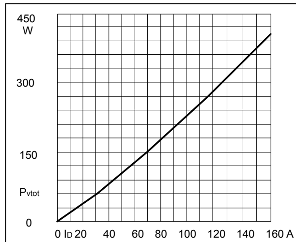
Fig2. Power dissipation
