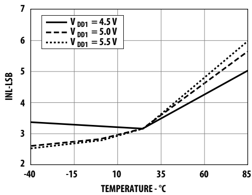
Figure 5. INL (Bits) vs. Temperature
