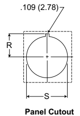
Panel Cutout
