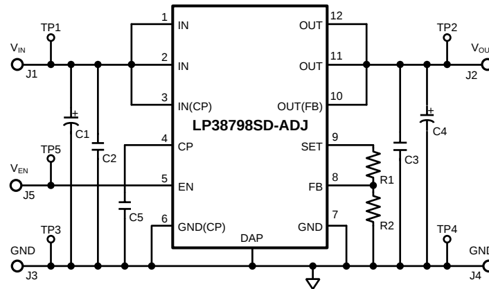
Figure 1. LP38798EVM Schematic
