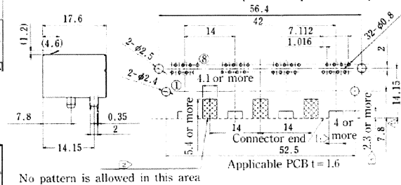
Reference mounting dimensions (PCB component side)
