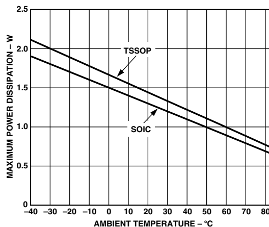
Figure 2. Plot of Maximum Power Dissipation vs. Temperature for AD8019 for T_J = 150^\circ\text{C}
