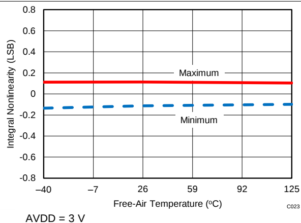
Figure 24. INL vs Free-Air Temperature
