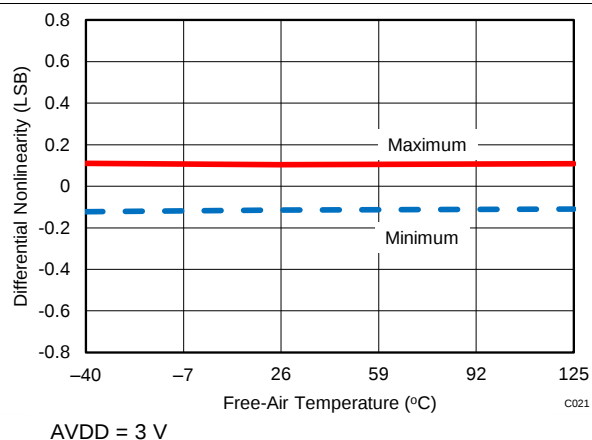
Figure 22. DNL vs Free-Air Temperature
